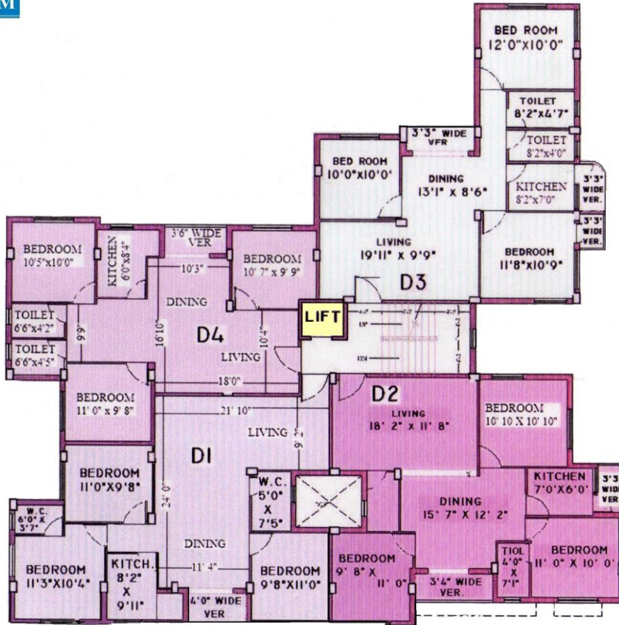
TYPICAL FLOOR PLAN (BLOCK-D)
